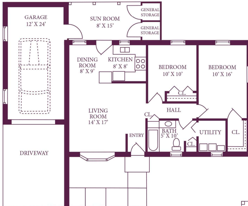
Cottage 2 Bedroom with Garage 1080 Square Feet
